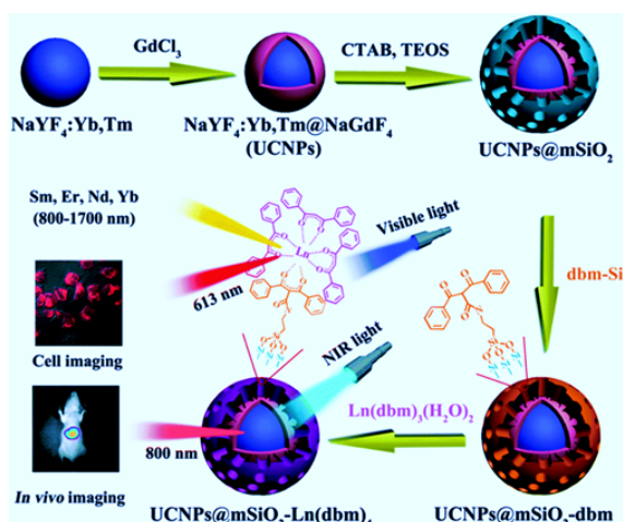
Figure. 1: Schematic of the preparation and structure of multifunctional mesoporous NPs containing both upconversion and magnetic nanophosphors (with an architecture of the type \text{NaYF}_4:\text{Yb,Tm}@ \text{NaGdF}_4 ) and covered with a conventional luminescent lanthanide complex ( \text{Ln}(\text{dbm})_3 ) for use in upconversion and downconversion luminescence imaging and as T1-weighted MRI contrast agents. From ref. 3
